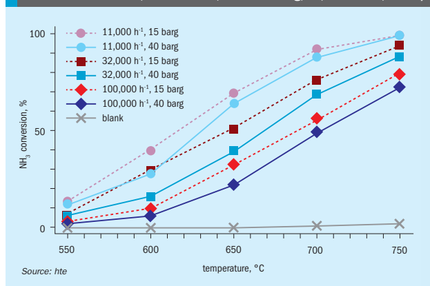
Fig. 2: \text{NH}_3 cracking over an Fe-based catalyst using hte's advanced high throughput technology (95% \text{NH}_3 , 5,000 ppm \text{H}_2\text{O} , Ar as balance and internal standard, 550 to 750^\circ\text{C} , 15 and 40 barg, 11,000 to 100,000 \text{h}^{-1} ).
