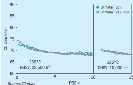
Fig. 3: High activity of ShiftMax 217 and ShiftMax 217 Plus
