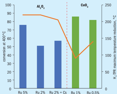
Fig. 1: NH 3 conversion measured at 400°C vs H 2 -TPR max. temp. reduction – for respectively Ru-Al 2 O 3 based catalysts (blue bars) and Ru-CeO 2 based catalysts (green bars).
