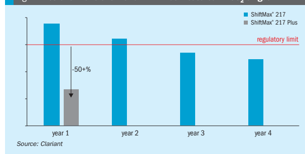
Fig. 4: Methanol make of ShiftMax 217 Plus measured in CO 2 off gas
