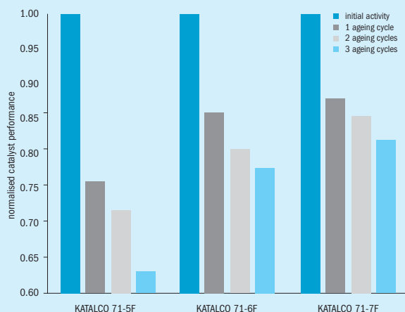
Fig. 4: Water gas shift catalyst performance for KATALCO HTS after representative thermal ageing
