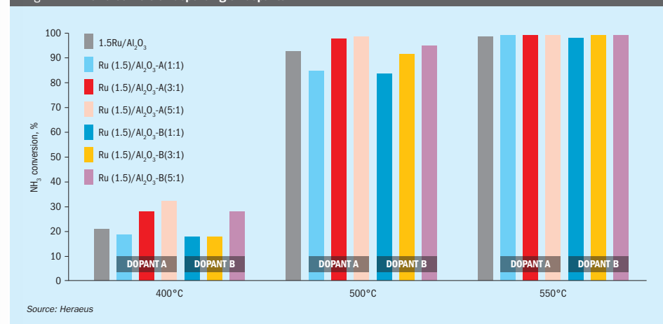
Fig. 1: Ammonia conversion depending on dopants
