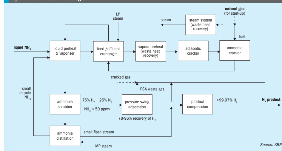
Fig. 1: H2ACT SM block flow diagram
