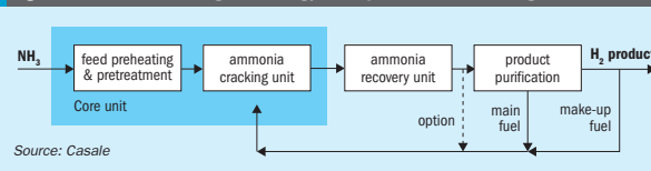
Fig. 1: Ammonia cracking technology – simplified self-sustaining scheme
