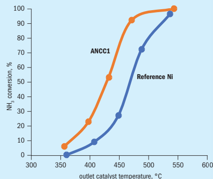
Fig. 2: NH 3 conversion (%) vs outlet cat. temp. (°C); [NH 3 ] inlet = 10% - SV = 10000h -1 - Atm.P.; reference Ni supported on alumina model coated catalyst (blue) vs base metal supported on rare earths oxides (ANCC1) (orange)
