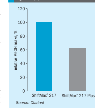
Fig. 1: By-product methanol formation
