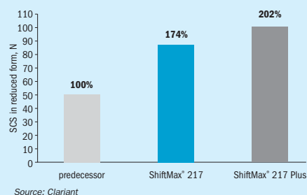
Fig. 2: Side crush strength after reduction
