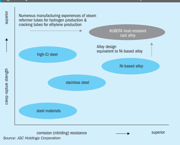
Fig. 1: Key characteristics and direction of tube metal development
