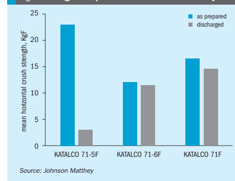
Fig. 2: Strength comparison for KATALCO HTS catalysts
