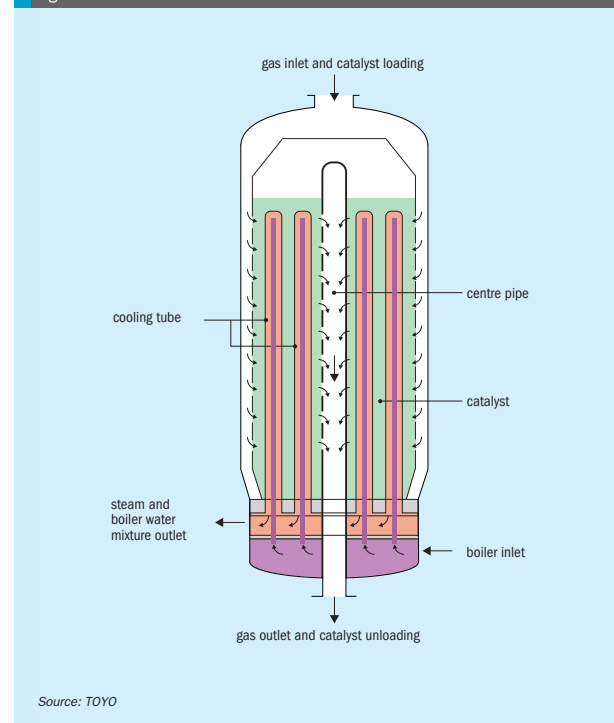
Fig. 6: MRF-Z® reactor
