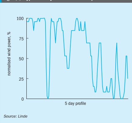
Fig. 5(a): Typical 5-day normalised wind power load curve
