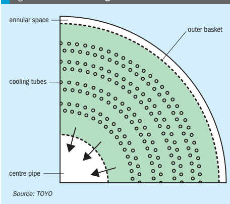
Fig. 4: MRF-Z® tube arrangement
