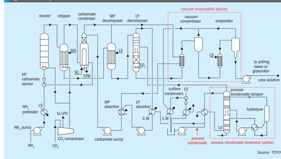
Fig. 1: TOYO urea process
