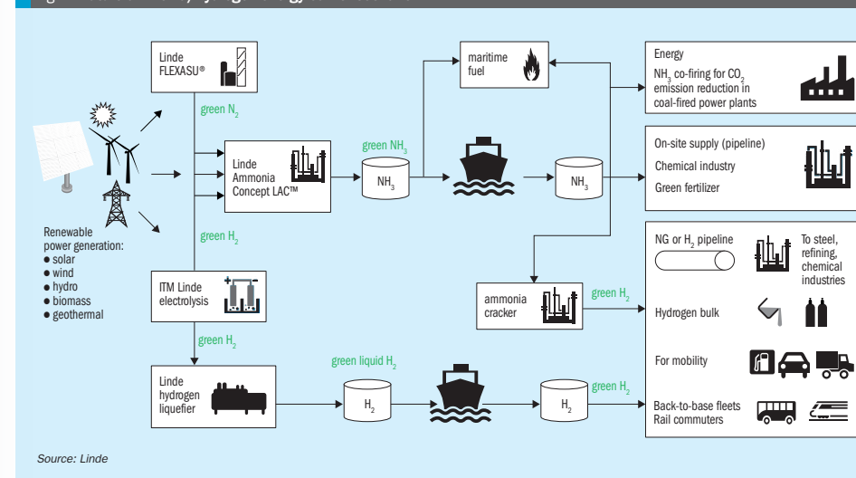
Fig. 2: Future ammonia/hydrogen energy carrier scenario
