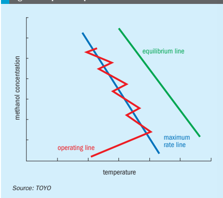
Fig. 5: Temperature profile
