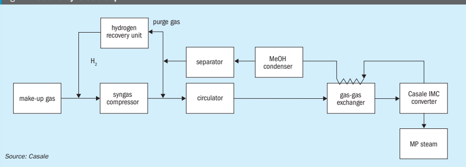
Fig. 4: Methanol synthesis loop
