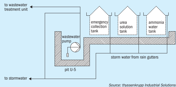
Fig. 3: Separation of oily wastewater from non-oily wastewater
