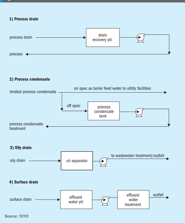
Fig. 5: Outline of wastewater treatment methods
