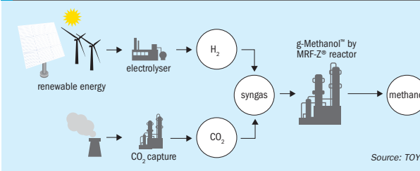
Fig. 2: g-Methanol® concept
