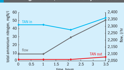
Fig. 5: Electrochemical system for total ammonium nitrogen removal, semi-industrial system results
