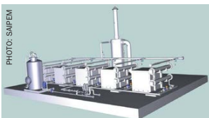
Fig. 7: 3D model of a SPELL plant.
