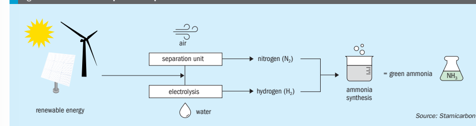
Fig. 2: “Green” ammonia production process
