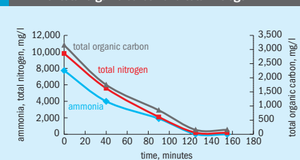
Fig. 3: Electrochemical system for simultaneous removal of total organic carbon and total nitrogen
