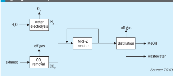
Fig. 3: g-Methanol® process flow scheme
