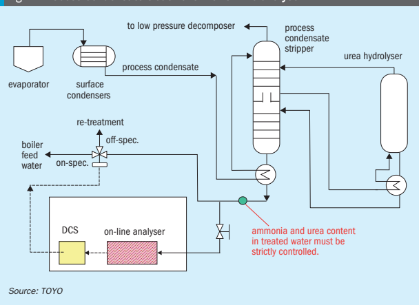
Fig. 2: Process condensate treatment with on-line analyser
