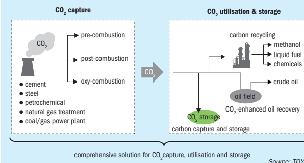
Fig. 1: TOYO CCUS Solution
