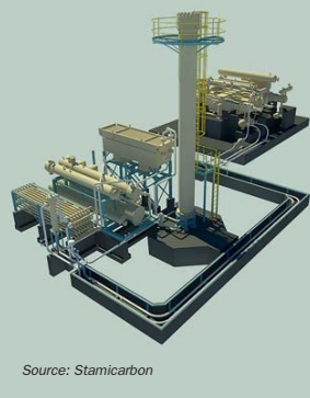
Fig. 3: 3D model of a Stami Green Ammonia plant
