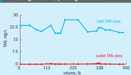
Fig. 4: Electrochemical system for total ammonium nitrogen removal, polishing treatment
