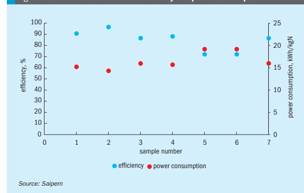
Fig. 1: Residual ammonia removal efficiency and power consumption
