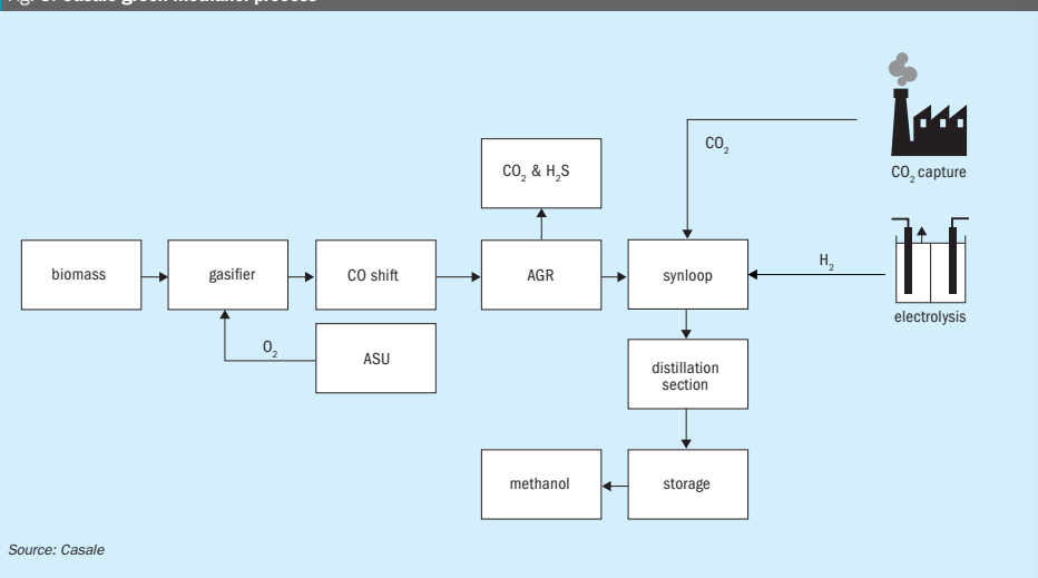
Fig. 3: Casale green methanol process
