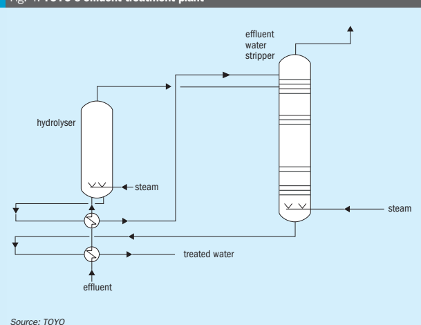
Fig. 4: TOYO's effluent treatment plant
