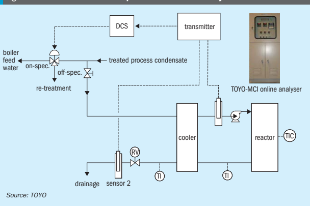
Fig. 3: Schematic flow of on-line process condensate analyser
