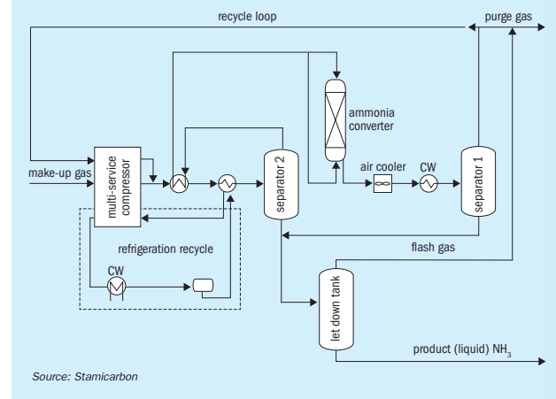
Fig. 4: Stami Green Ammonia technology
