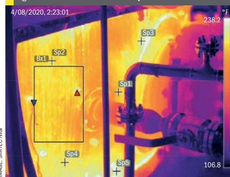
Fig. 8: WHB rear channel skin temperature measurement
