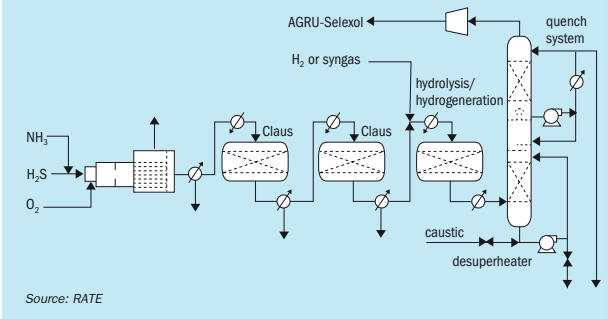
Fig. 2: The sulphur recovery unit
