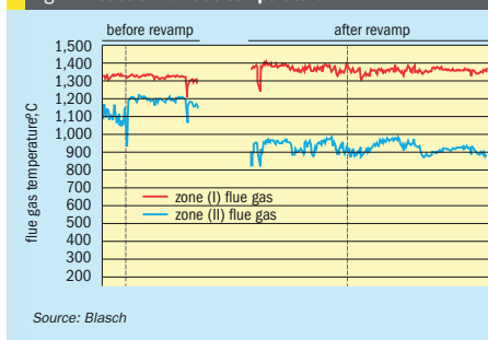
Fig. 2: Reaction furnace temperature
