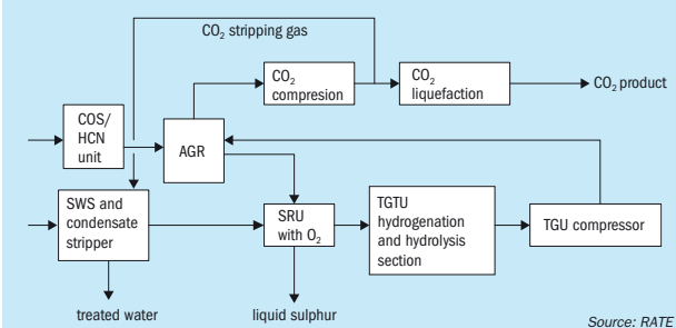
Fig. 2: The sulphur recovery unit
