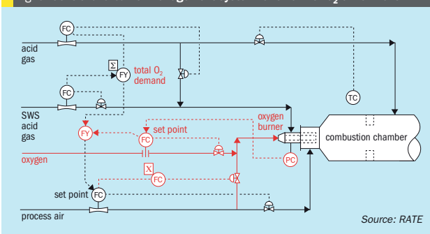
Fig. 3: Control and burner management system for SRU with O 2 enrichment
