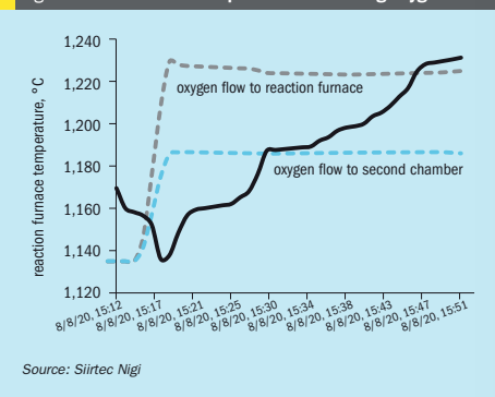
Fig. 9: Thermal reactor temperature trend during oxygen cut-in
