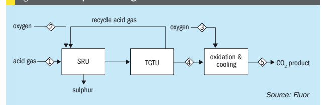
Fig. 1: One of the process configurations of OEC 2 RP
