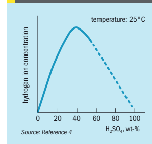
Fig. 1: Acid composition affects the concentration of hydrogen ions in H_2SO_4
