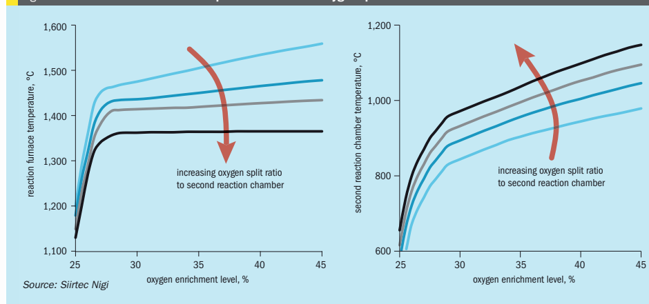
Fig. 10: Overall enrichment versus temperature at different oxygen split ratios
