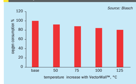
Fig. 3: Oxygen optimisation with VectorWall™ temperature enhancement
