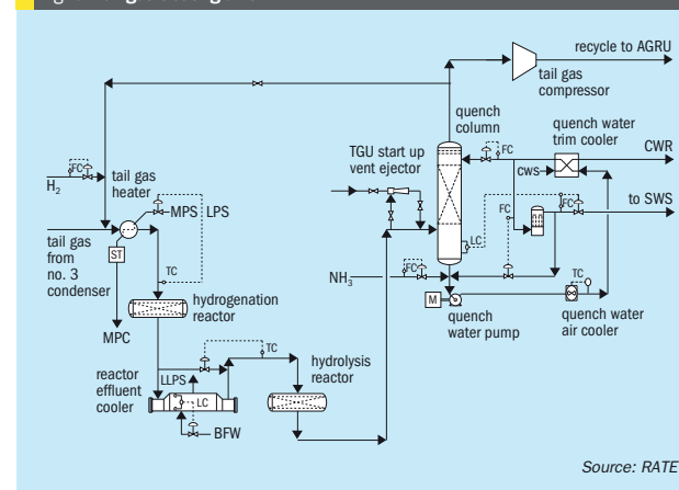
Fig. 5: Tail gas treating unit
