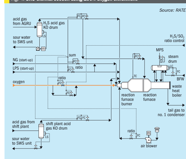
Fig. 4: SRU thermal section using 100% oxygen enrichment
