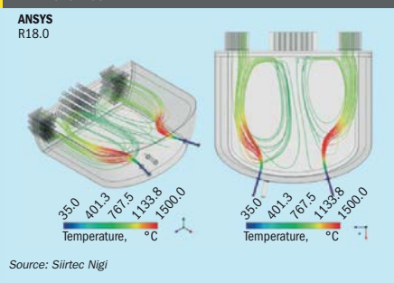
Fig. 6: CFD temperature streamlines in second combustion chamber
