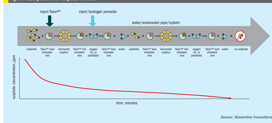
Fig. 3: TSES process for sulphide removal
