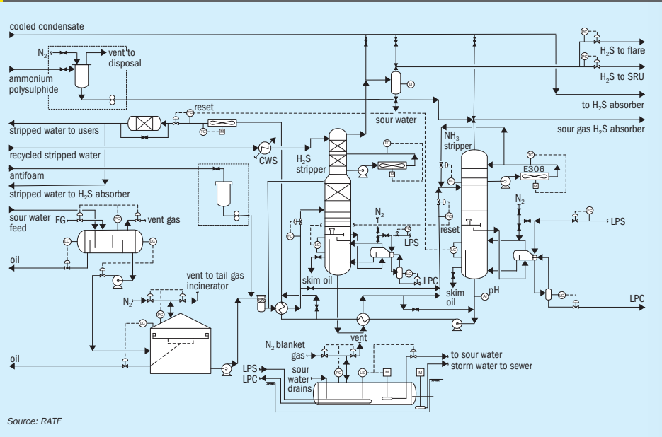
Fig. 3: RATE two-stage SWS-MAX sour water stripping
