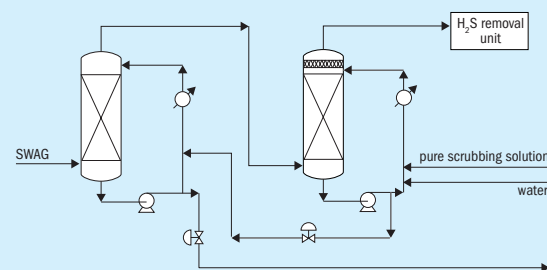
Fig. 4: Process flow scheme for acidic removal of ammonia prior to sulphur scavenging unit
