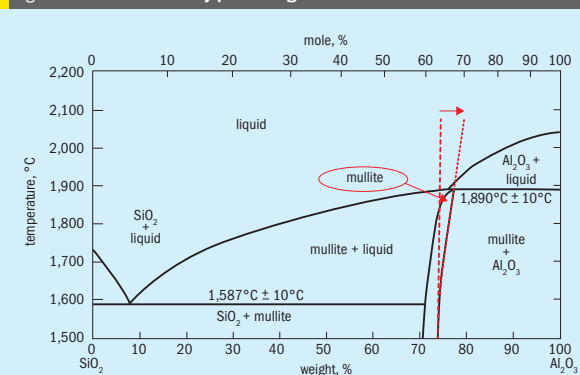
Fig. 1: Alumina-silica binary phase diagram
