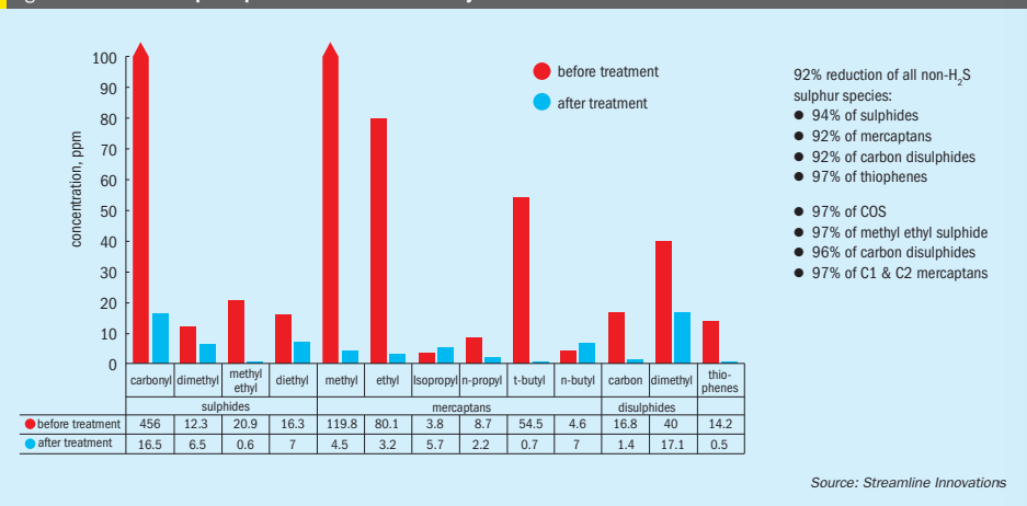
Fig. 1: Reduction of sulphur species in a direct treat Valkyrie™ unit
