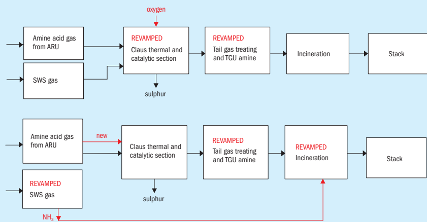
Fig. 5: SRU capacity expansion options
