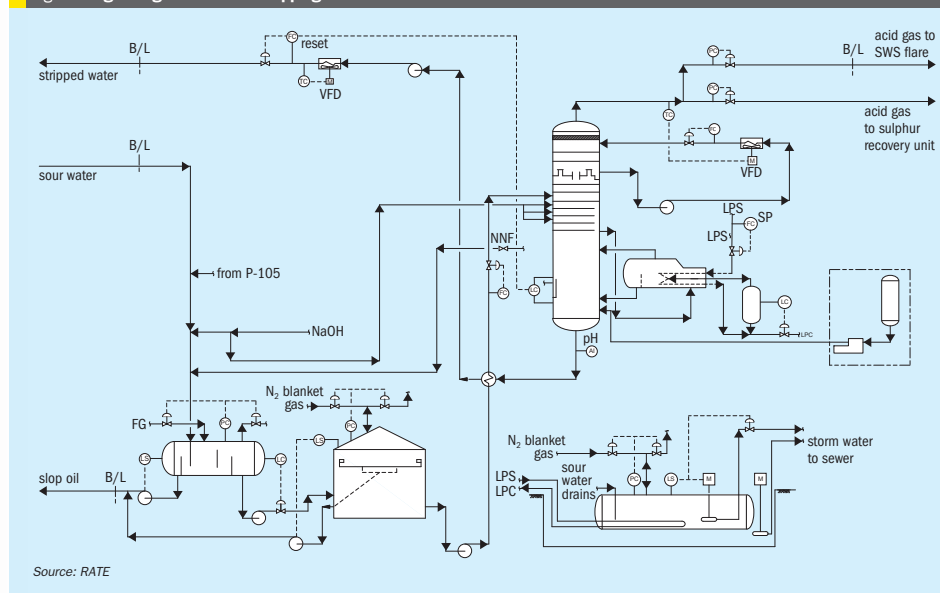
Fig. 1: Single-stage sour water stripping
