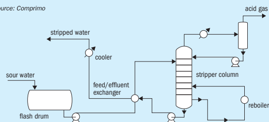
Fig. 1: Process flow scheme of single-stage sour water stripper
