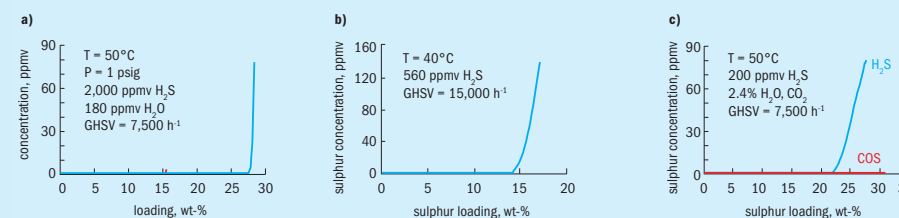
Figs 4(a-c): H 2 S breakthrough profile for treatment of (a) dry natural gas over the SulfaTrap™-R7J sorbent, (b) LPG over the SulfaTrap™-R7J sorbent, (c) wet natural gas over the SulfaTrap™-R7Q sorbent
