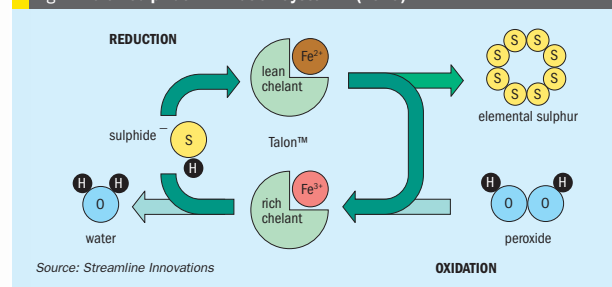
Fig. 2: Talon Sulphide Elimination System™ (TSES)
