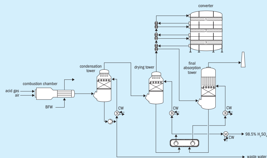
Fig. 1: Process flow diagram for thyssenkrupp Uhde's alternative sulphuric acid process – strong acid from wet acid gas
