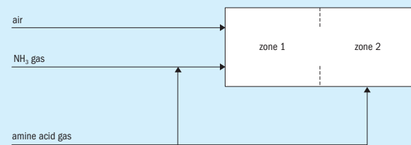
Fig. 6: Two-zone reaction furnace
