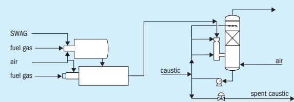
Fig. 3: Process flow scheme for ammonia burning thermal oxidiser with scrubber
