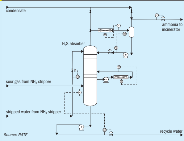
Fig. 4: RATE two-stage SWS-MAX sour water stripping
